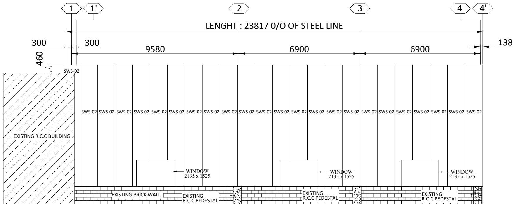
SIDE WALL SHEETING @ GRID - A
