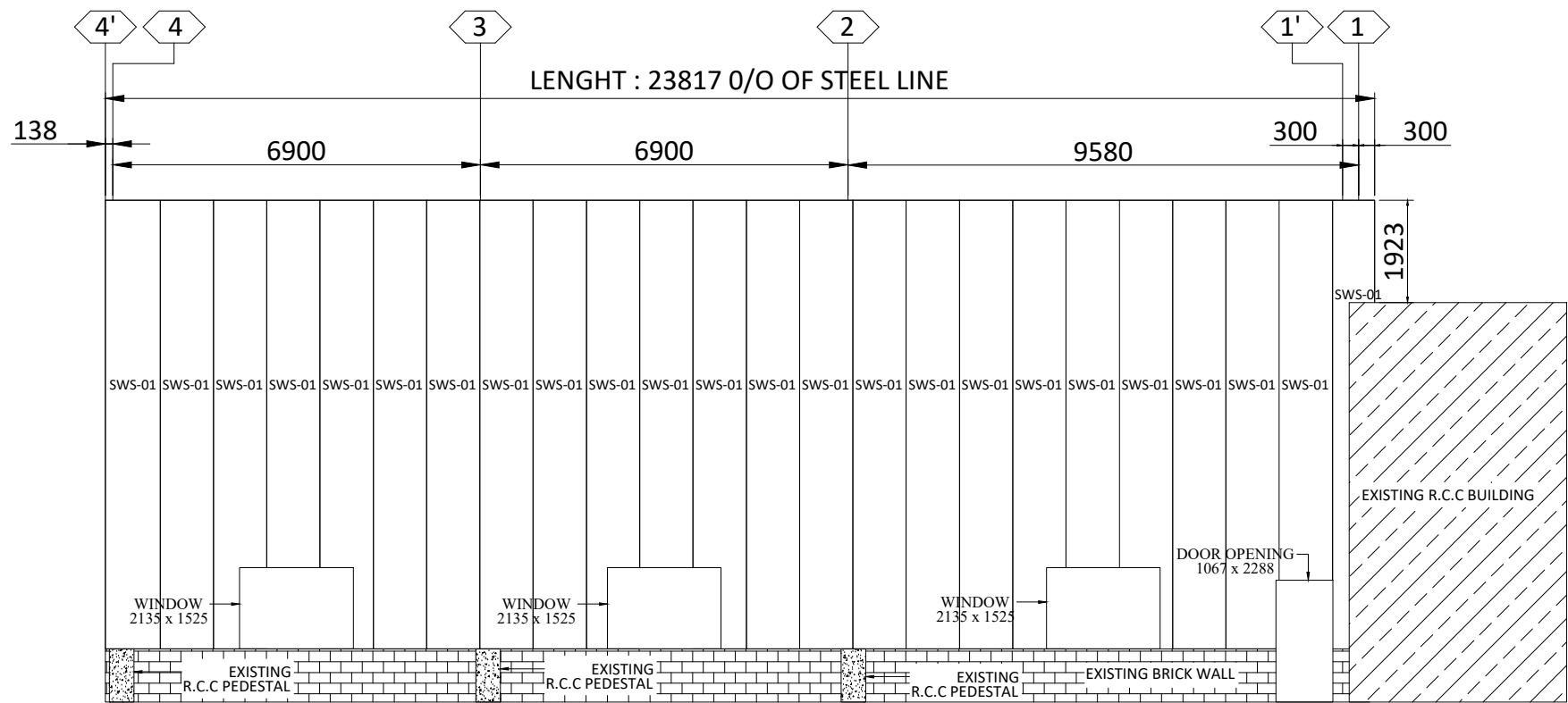
SIDE WALL SHEETING @ GRID - A
